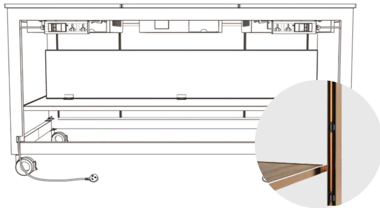
Open wire slot
